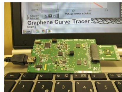
Figure 4: LoC made of (from right to left) a 22 graphene transistor chip wire-bonded to the printed circuit board, which is inserted in a connector transmitting the signals from/to the integrated control electronics board, connected to the PC via a USB cable.
